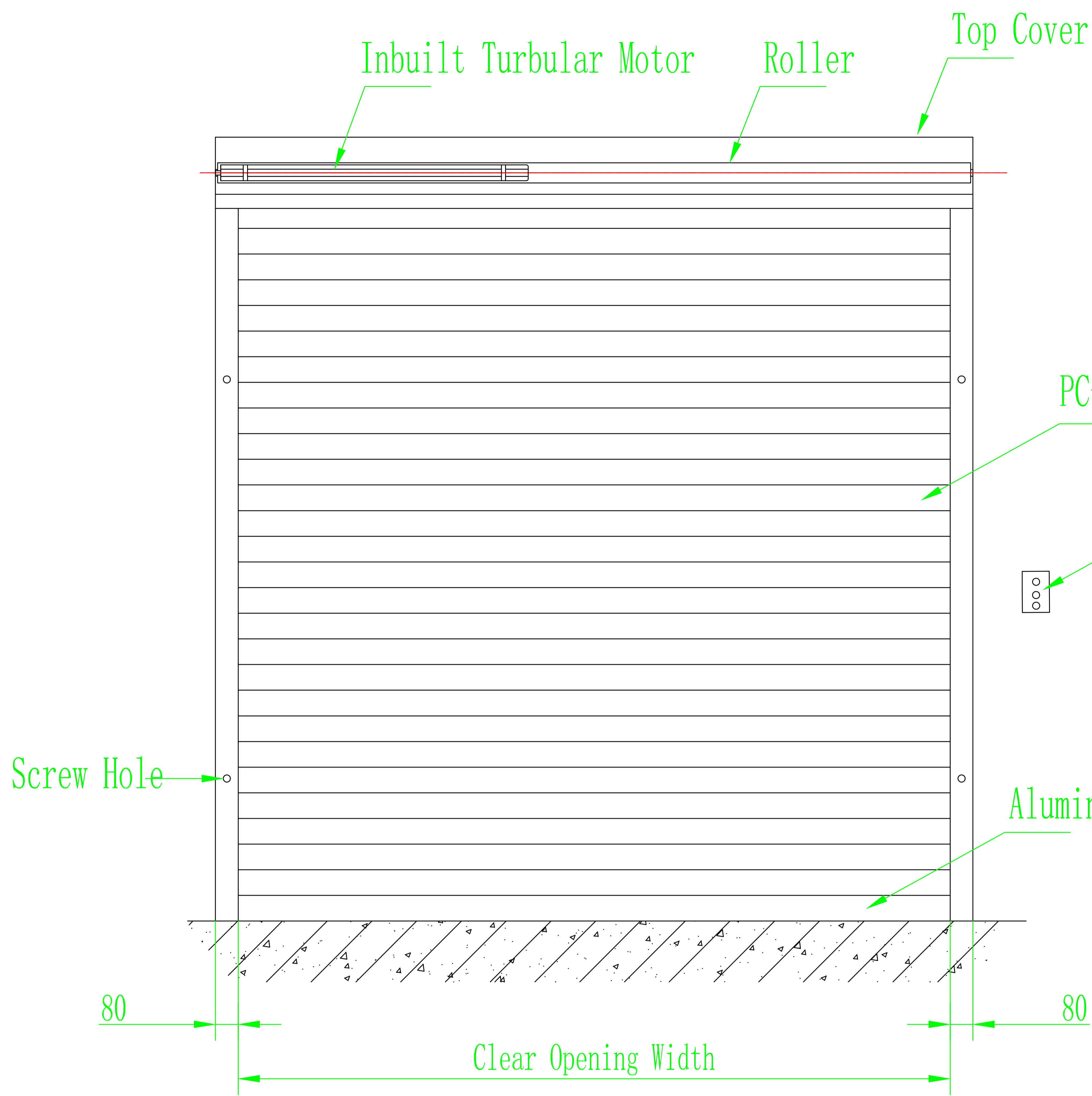
ELEVATION VIEW
