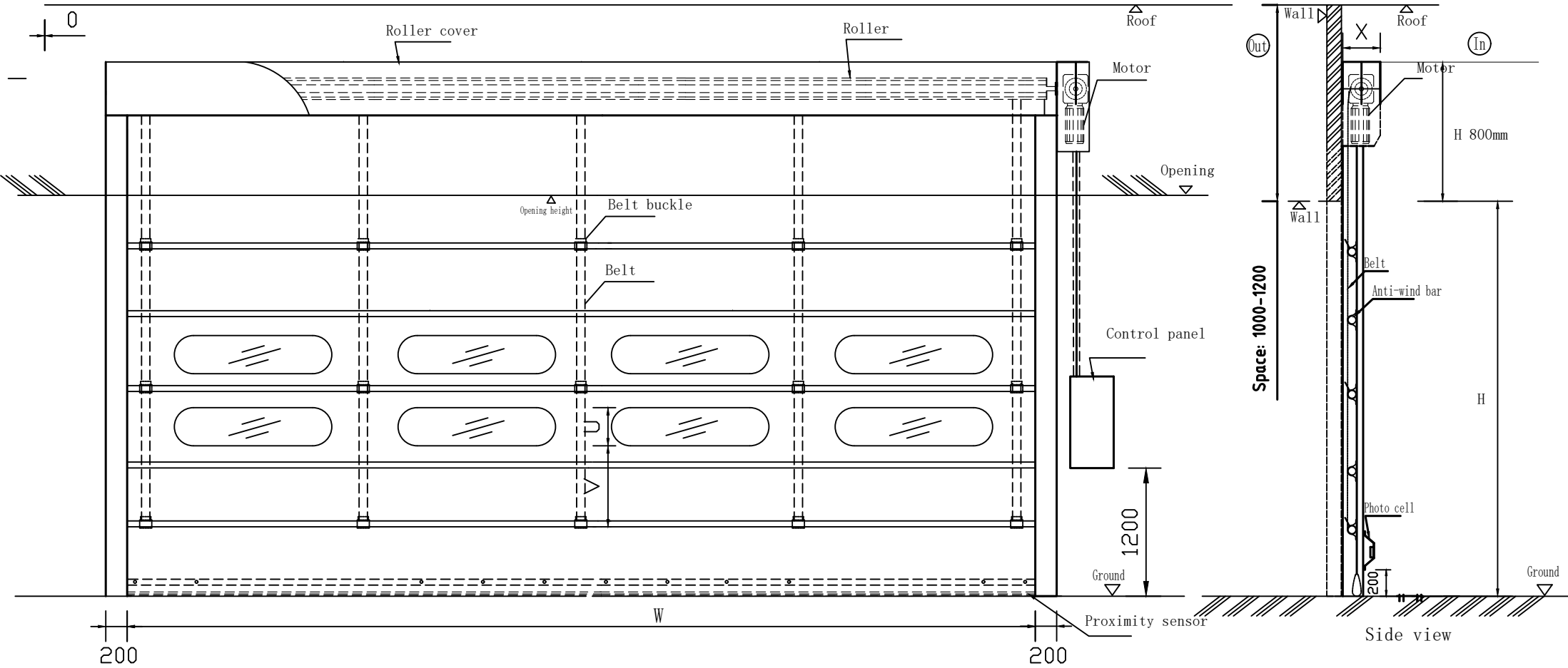
Front view
